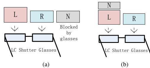
Figure 2: (a) In the three frame method, a third channel is inserted to display the [Neither] image. (b) A two frame approximation can be achieved by adding the [Neither] image to the [Left] image.
